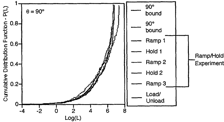
Figure 10. CDF of AE events detected from all 90° samples with L as the distribution parameter. Data bounds collected from the rate testing are shown by the dotted lines. Data from ramp/hold testing has been broken into separate pieces so cracking from each segment is easily viewed.
