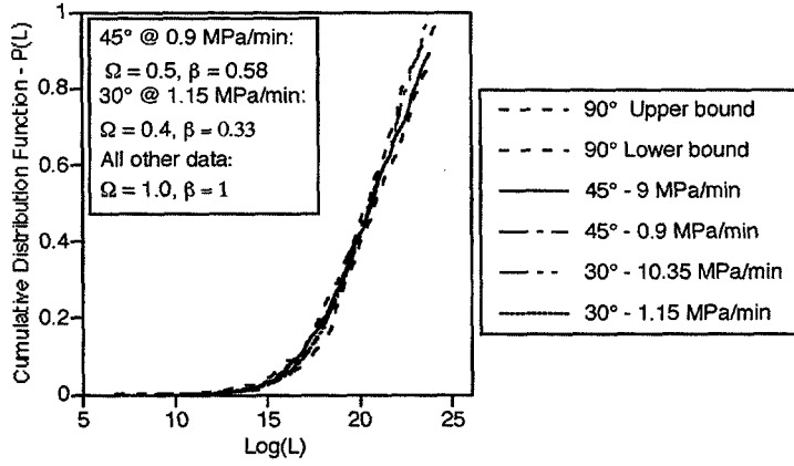
Figure 11. CDF of AE events detected from off-axis and 90° samples loaded with different rates with L as the distribution parameter.
