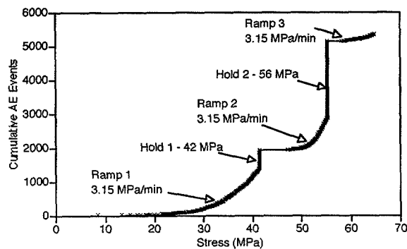
Figure 7. Cumulative AE events versus stress detected during ramp/hold testing of a 90° sample. Testing was performed with B225 sensors.
