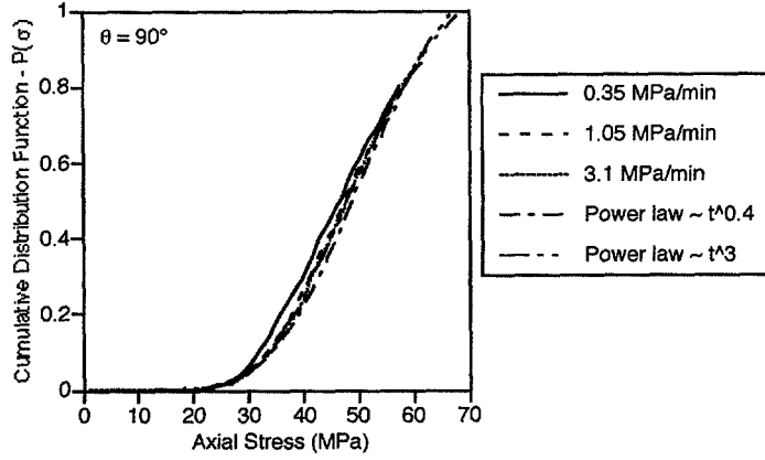
Figure 9. CDF of AE events detected from 90° samples loaded with different histories when using axial stress as the distribution parameter. Each curve represents the average of multiple cycles.
