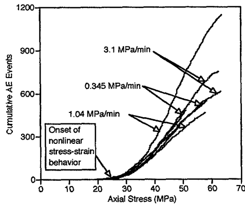
Figure 6. Cumulative AE events detected in 90° samples versus axial stress for three loading rates.
