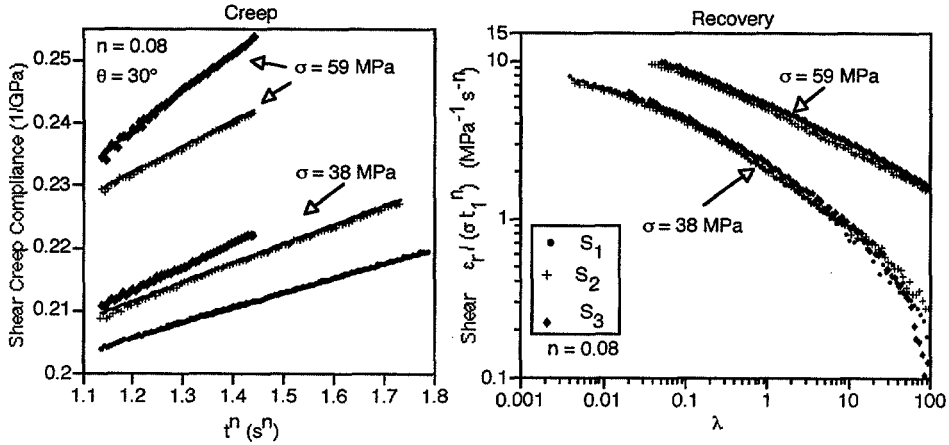
Figure 3. Shear creep compliance of a 30° off-axis sample at 38 MPa and 59 MPa for three damage states. Damage states S_1 and S_2 were cycled 9 times for 100s at each stress. Damage state S_3 is from a single 100s cycle.
