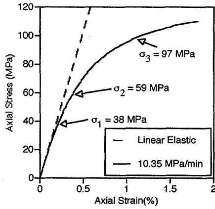
Figure 2. Stress strain response of 30° samples with the stresses used in the damage effect study.
