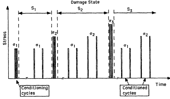
Figure 1. Generic loading history for conducting a damage effect study. Duration of each creep cycle is the same. Three damage states are shown, designated by S_i corresponding to conditioning at \sigma_i .
