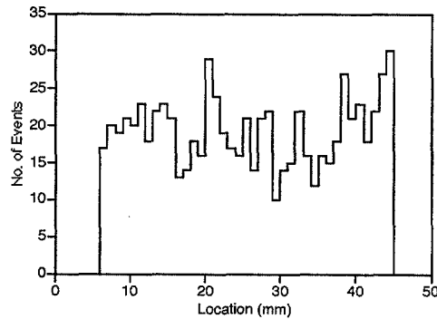
Figure 5. Histogram of cracking in the free length of a 90° sample. Events shown are between the AE sensors in a uniformly stressed portion of the material. Specimen gage length was approximately 17 cm.
