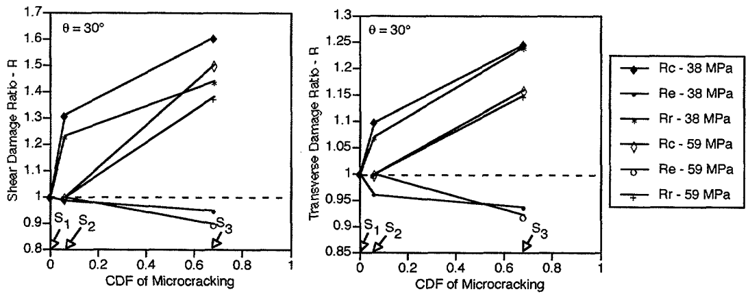
Figure 4. Shear compliance damage effect ratios from a 30° sample. A damage state has been characterized by the Cumulative Distribution Function of microcracking at that state. Estimates for the value of the CDF were made from ramp testing data using AE monitoring.
