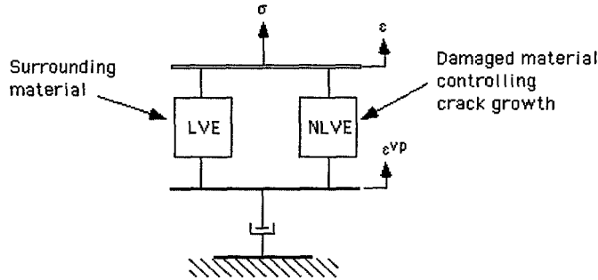
Figure 8. Idealized mechanical analog of the material containing a nonlinear viscoelastic phase in the vicinity of crack tips (driving the crack growth) surrounded by a linear viscoelastic material. A viscoplastic component has also been added to be consistent with experiments.
